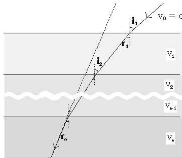
Figure 25: Atmospheric refraction.
